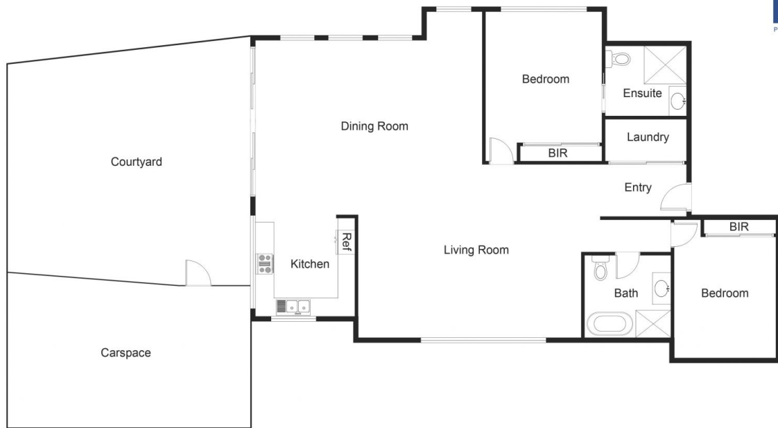
FLOOR PLAN
